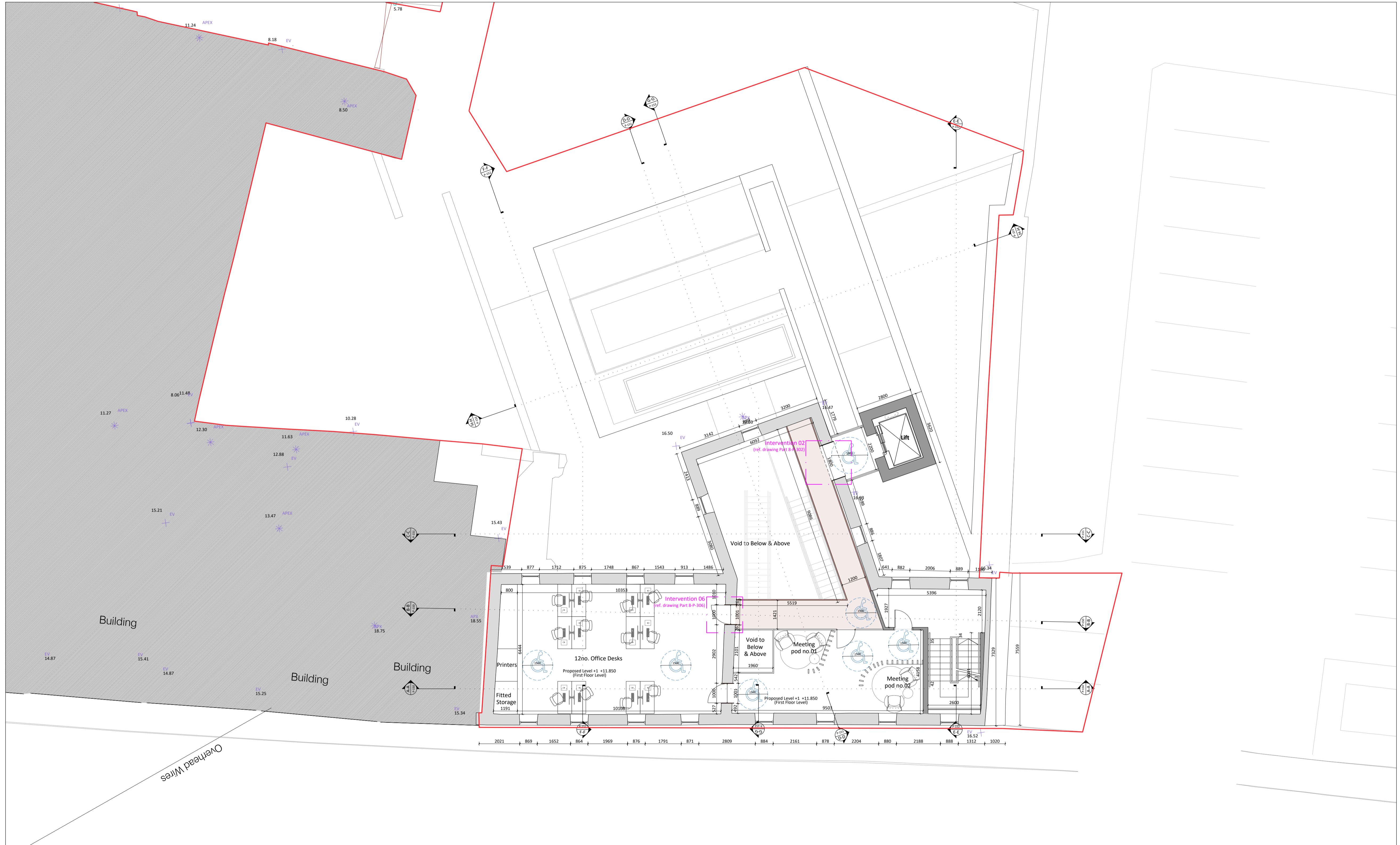
01 Level 1 (First) Floor Plan As Proposed Scale: 1:100
